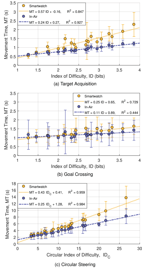
Figure 7: Across-participants, mean movement time MT versus index of difficulty ID . Error bars show \pm 1 standard deviation.
