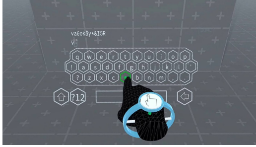
(a) INDEXPOINT-0: Typing on the primary alphabetic character layer.
