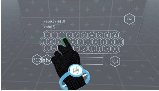
(c) INDEXPOINT-180: Typing on the tertiary symbol and punctuation layer.
