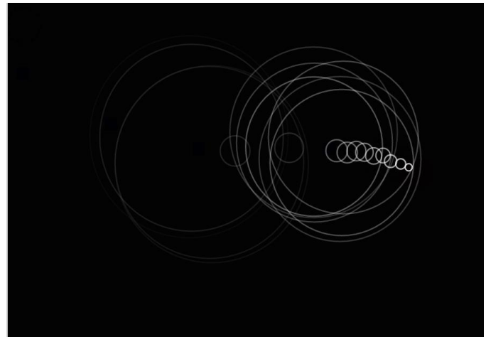
Fig. 3: The application shows an object moving along a fixed trajectory (left). When the display is unattended it is automatically dimmed to reduce operator distraction using an event rule (right). In the dimmed display, delta changes in the underlying application are made available to the operator's peripheral vision by being visualised using an information filter.
